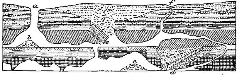
FIGURE 15.—Sketch section illustrating the formation of solution caverns in strata containing gypsum and rock salt. The caverns are formed in the gypsum and rock salt, and connecting channels are cut through the limestone and other strata. At the bottom of opening a is some of the material b which fell from the roof; at c material which fell within the cavern; at d and e masses of hard rock which slumped when support was removed from one side; at f a small choked opening; at g an old sealed opening.
