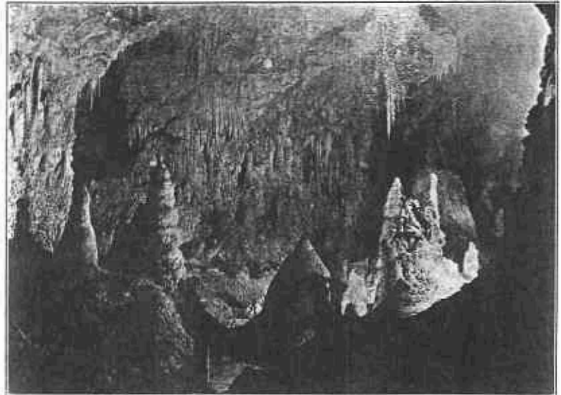
B. A CHARACTERISTIC SCENE IN CARLSBAD CAVERN.
